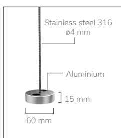
Cord Guiding
