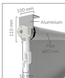
Head Rail
