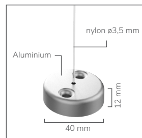
Cord Guiding
