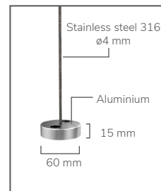
Cord Guiding
